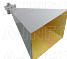
LB-284-20-C-7/16F Standard Gain Horn Antenna 2.6-3.95GHz 20dB Gain 7/16(DIN) Female
