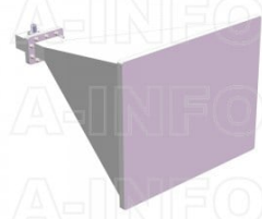
LB-284-20-C-NFSPS Standard Gain Horn Antenna 2.6-3.95GHz 20dB Gain N Type Female
